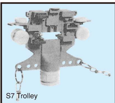
Trolley guide roller
